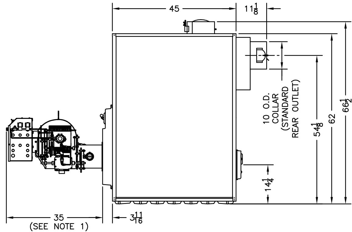
RIGHT SIDE VIEW (BURNER INSTALLED)
