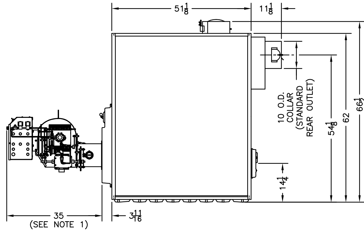
RIGHT SIDE VIEW (BURNER INSTALLED)
