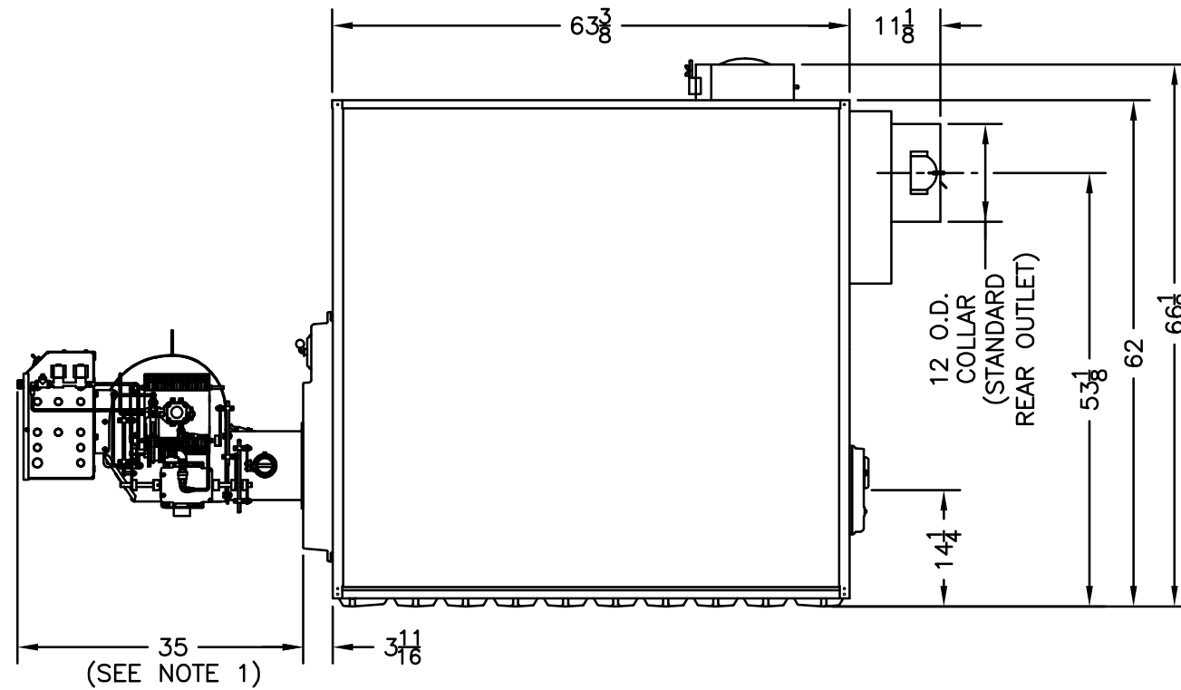
RIGHT SIDE VIEW (BURNER INSTALLED)
