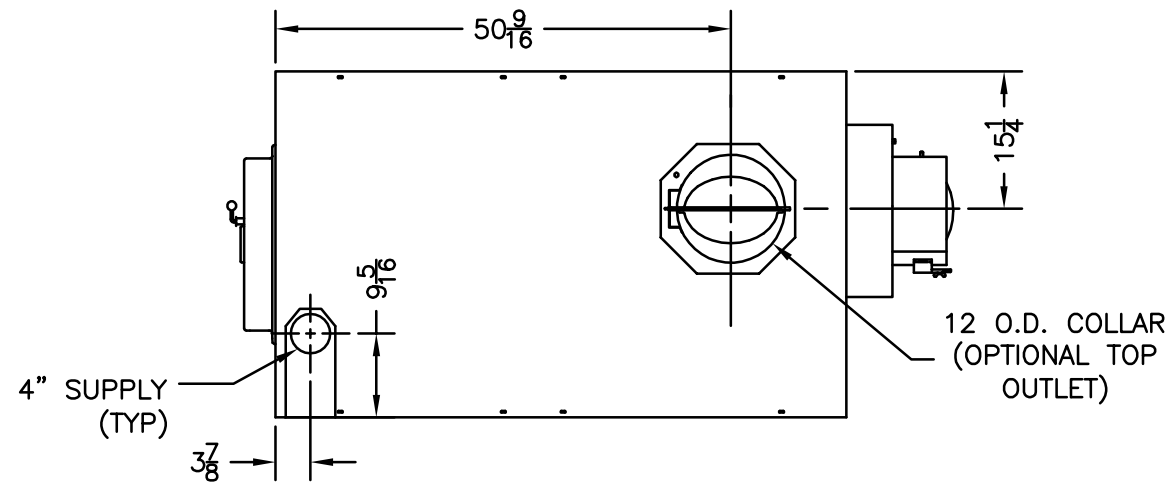
TOP VIEW
