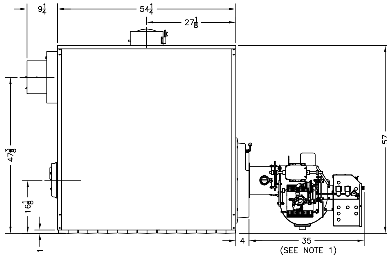
LEFT SIDE VIEW (BURNER INSTALLED)
