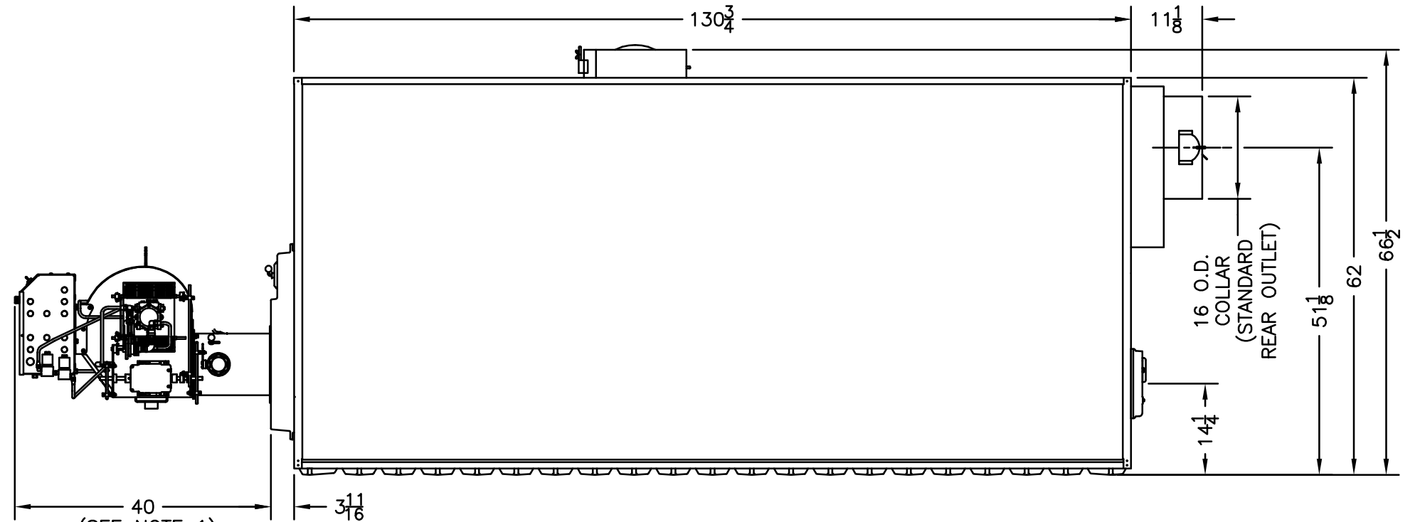
RIGHT SIDE VIEW (BURNER INSTALLED)
