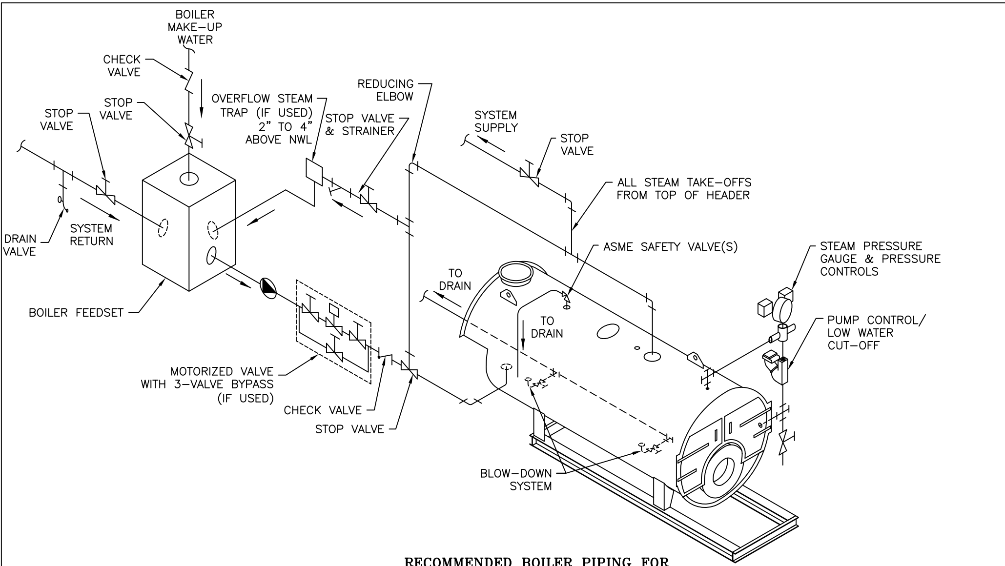
RECOMMENDED BOILER PIPING FOR SINGLE LOW PRESSURE SCOTCH STEAM BOILER WITH PUMPED RETURN
