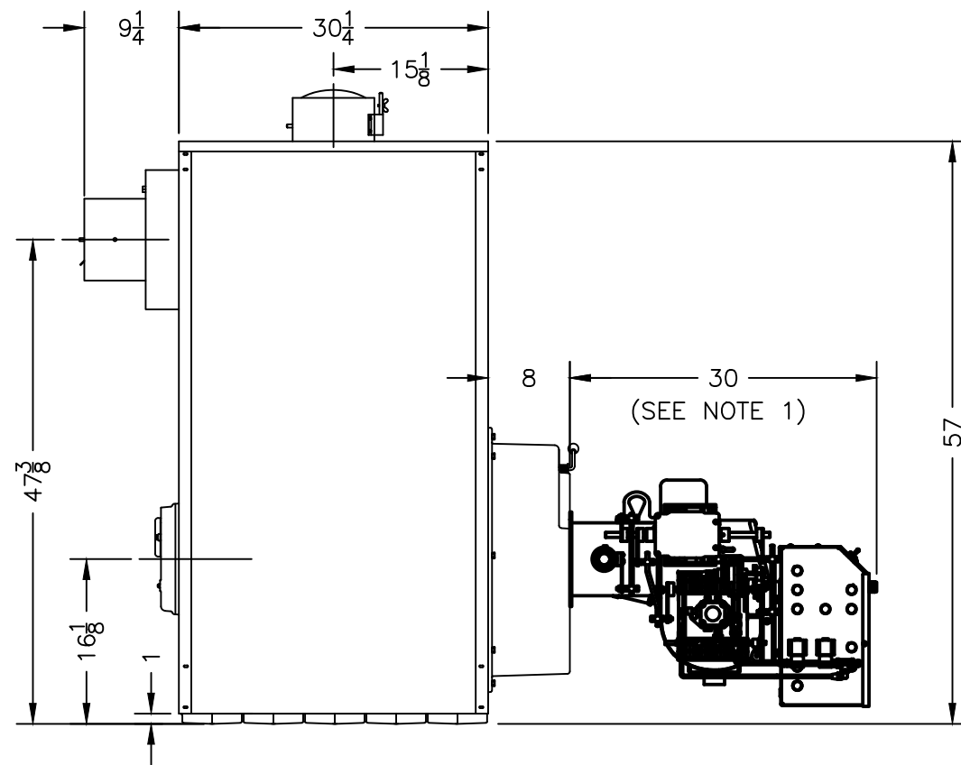
LEFT SIDE VIEW (BURNER INSTALLED)
