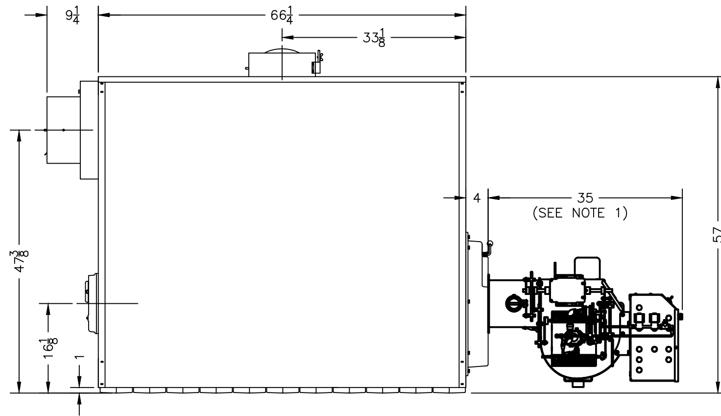
LEFT SIDE VIEW (BURNER INSTALLED)
