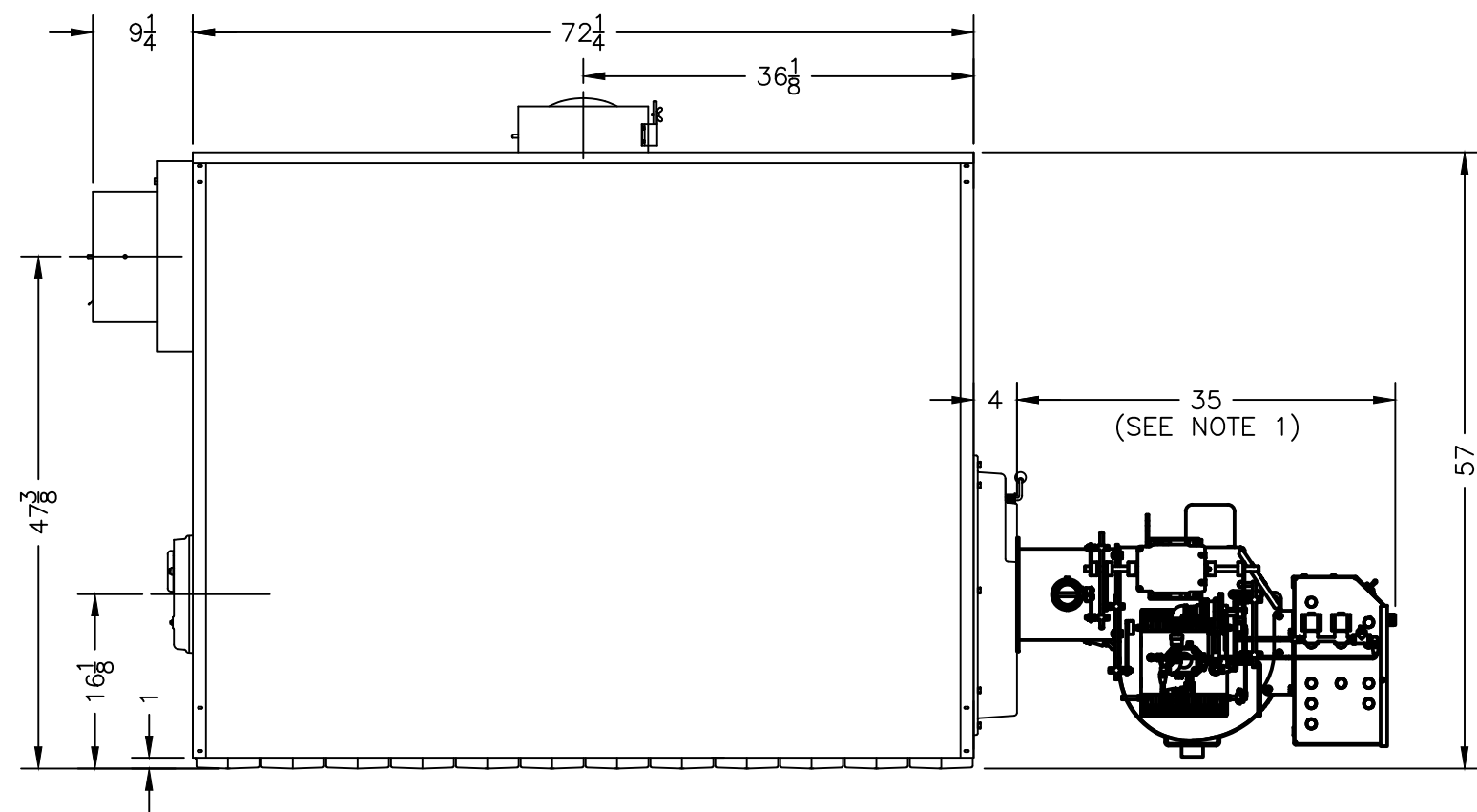
TOP VIEW
