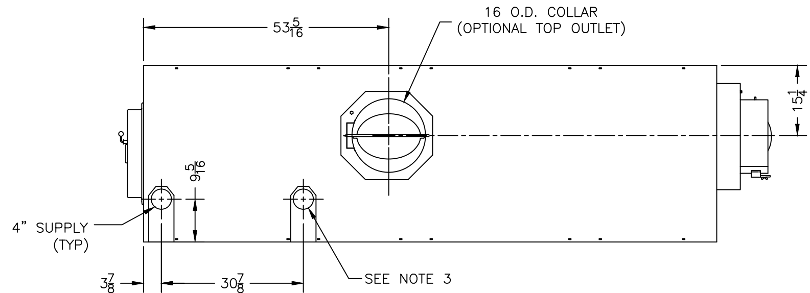
TOP VIEW
