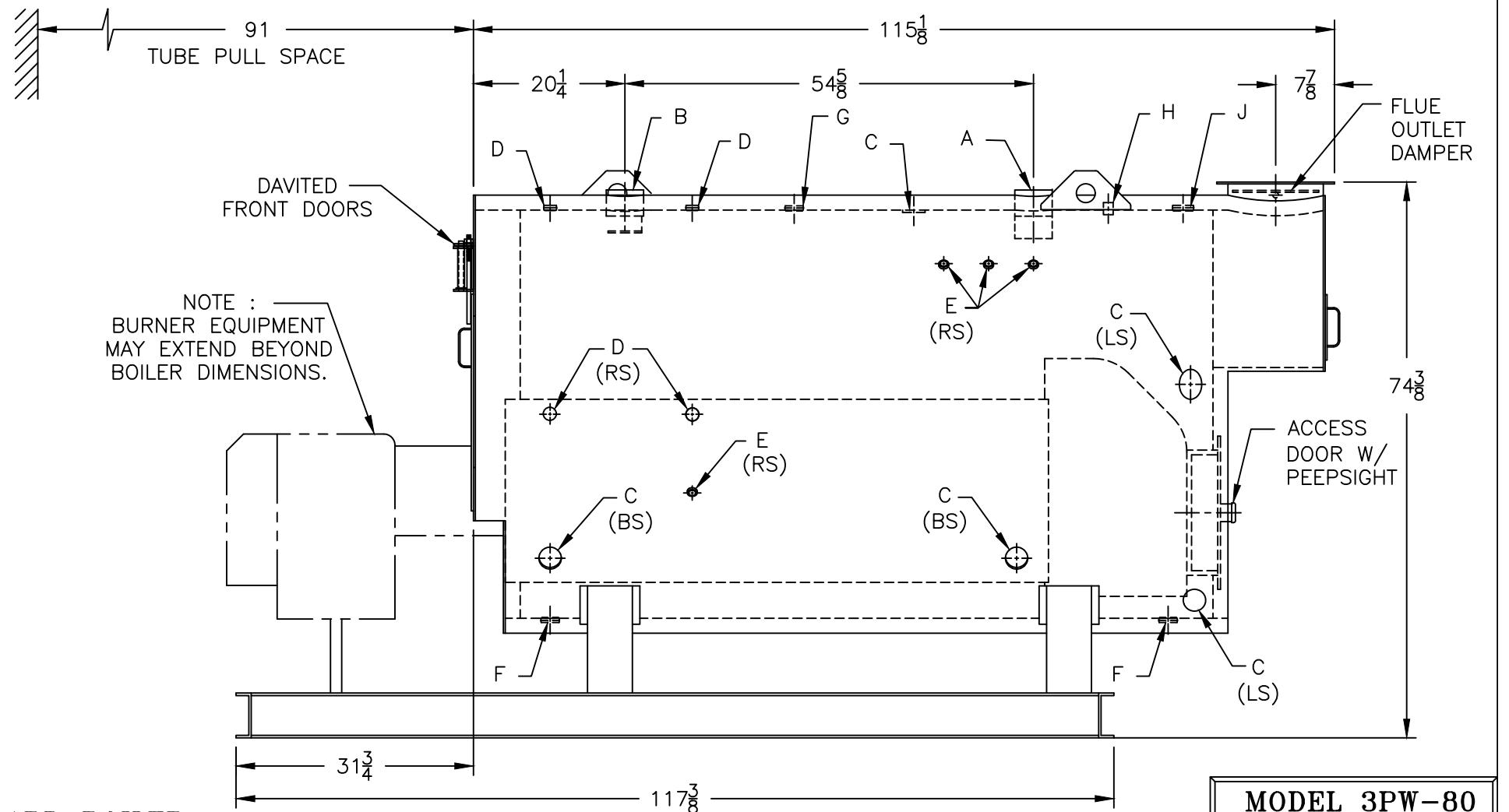
PROJECT: STANDARD BOILER
